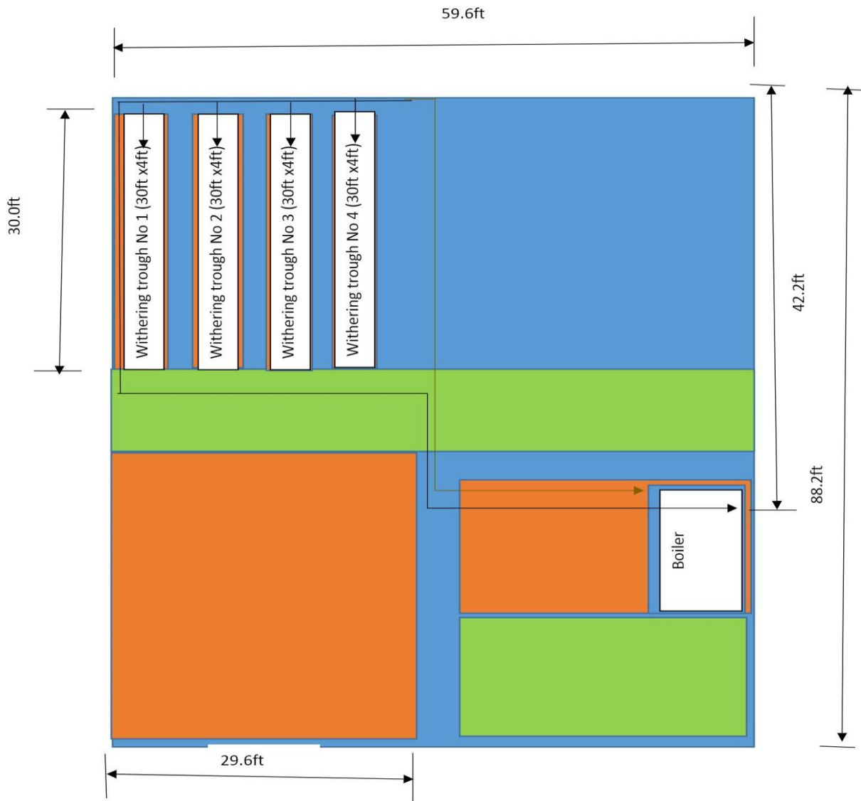
Schematic Diagram for boiler and withering troughs pipes layout
